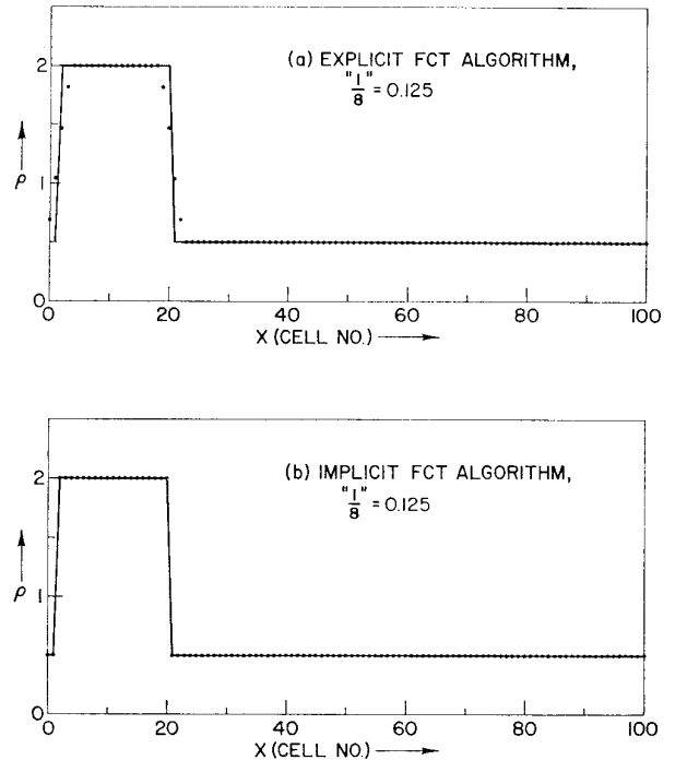
FIG. 11. Same comparison as Fig. 10 except the flow velocity is zero. The solid line again shows the correct solution. Here the implicit FCT algorithm (b) gives the exact answer whereas the somewhat simpler explicit method still has a small residual smoothing.
