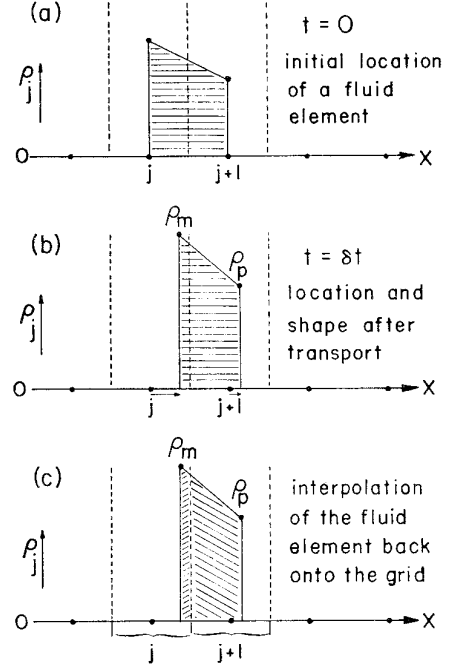
FIG. 1. The transport stage of the 1 D FCT algorithm SHASTA (Stage 1). Linear interpolations are used throughout so that mass is conserved and the density is nonnegative as long as |v\delta t/\delta x| < \frac{1}{2} .
