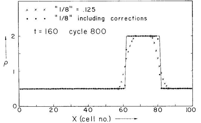
FIG. 4. Comparison of the 1 D FCT algorithm SHASTA with and without k - and v -dependent corrections to the antidiffusion coefficient. Notice the improvement obtained even by the simple formulation “ \frac{1}{8} ” = 0.125 in comparison with the standard schemes of Fig. 3.
