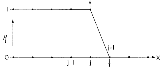
FIG. 2. Showing the non-sign-preserving tendencies of antidiffusion. At gridpoint j a new maximum will be created by antidiffusion and the new minimum at j + 1 will be negative.
