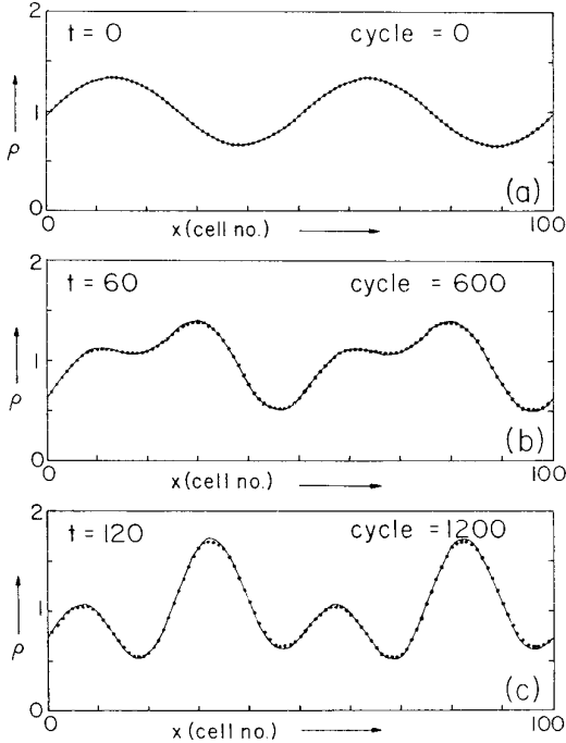
FIG. 5. A test of SHASTA on a problem where new maxima and minima appear physically. Mode 2 is excited initially using an analytic time- and space-dependent velocity and Mode 4 grows with time. The weak clipping phenomenon at maxima and minima is a result of the simple flux-limiting correction of Stage II.
