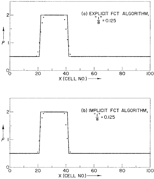
FIG. 10. Comparison of simple explicit (“ \frac{1}{8} ” = 0.125) and simple implicit versions of FCT antidiffusion using the SHASTA transport algorithm. The velocity is unity and \varepsilon = 0.2 . The time is t = 20 (cycle = 100). The implicit FCT antidiffusion is marginally better than the explicit version and both are far better than the standard schemes of Fig. 5.
