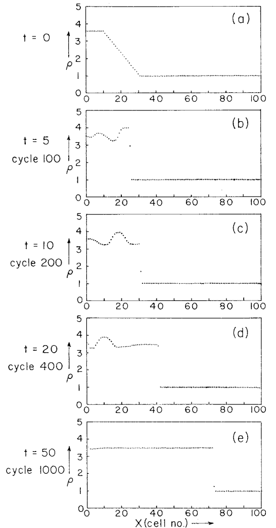
FIG. 6. Evolution of a ramp initial condition into a strong shock. The ramp transient in density, velocity, and pressure leaves sound waves propagating away on the downstream side of the shock. The correct Rankine-Hugoniot conditions are rapidly achieved.
